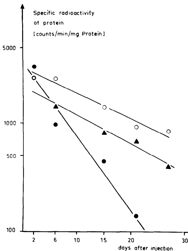
Fig. 2. Changes of the specific radioactivity of mitochondrial subfractions with time. \bullet — \bullet outer membrane, \circ — \circ inner membrane, \blacktriangle — \blacktriangle soluble protein. Ordinate in logarithmic scale.
