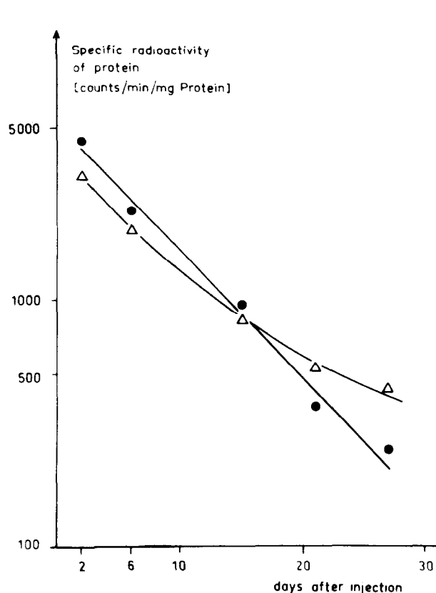
Fig. 1. Changes of the specific radioactivity of mitochondrial \Delta — \Delta and microsomal \bullet — \bullet proteins with time. Ordinate in logarithmic scale.
